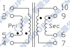
SCHEMATICS 2
