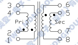
SCHEMATICS
