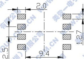
LAND PATTERN
