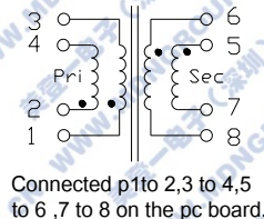
SCHEMATICS
