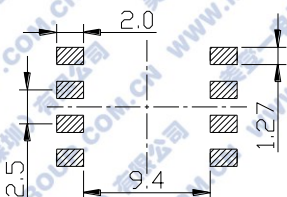
LAND PATTERN
